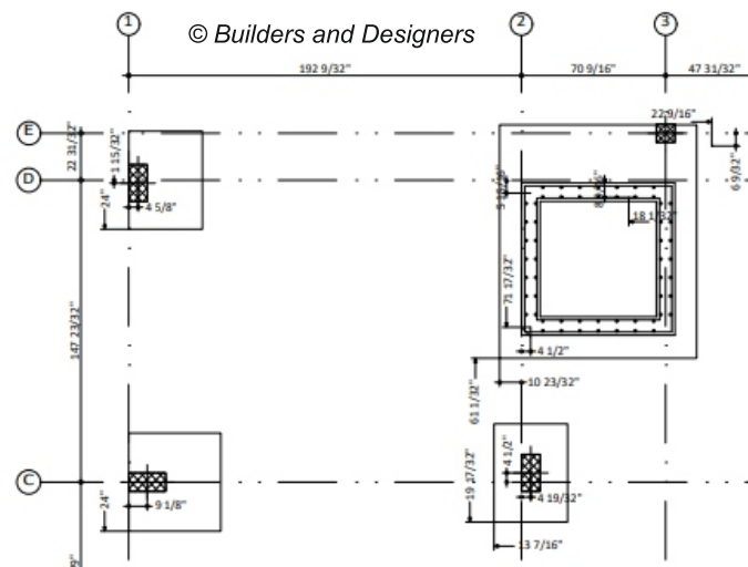
Structural Design of Residential Building prepared for Mr. Habeeb ur Rahman, Site No. 95, Balajee Layout, Hegde Nagar, Phase III, Bangalore
