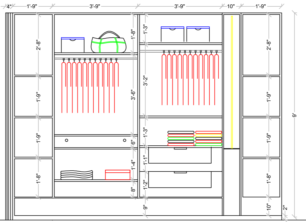
ELEVATIONS
