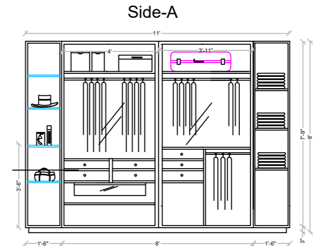
ELEVATIONS SON'S WARDROBE 1st FLOOR, Interior
