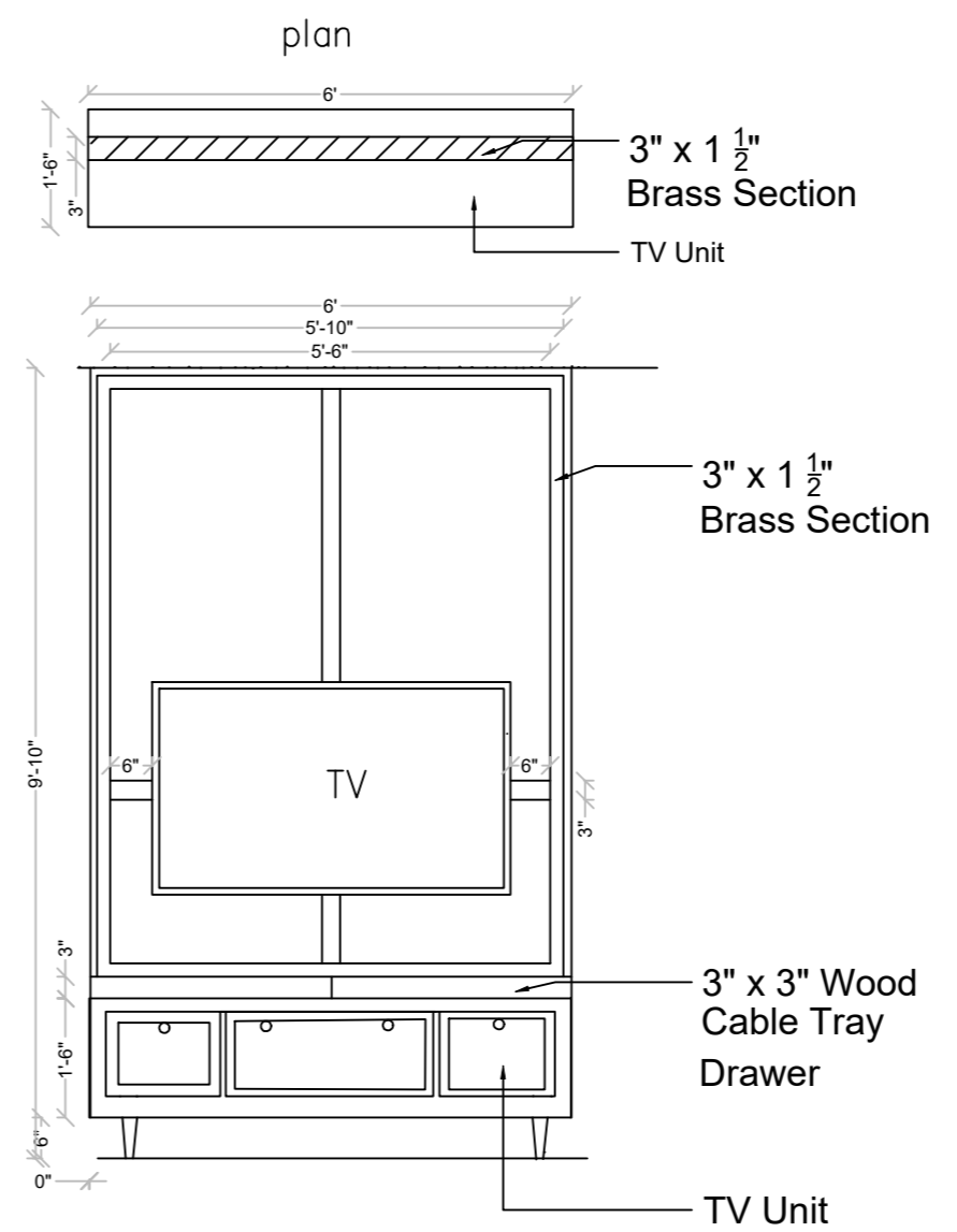
TV Unit , Dining side
