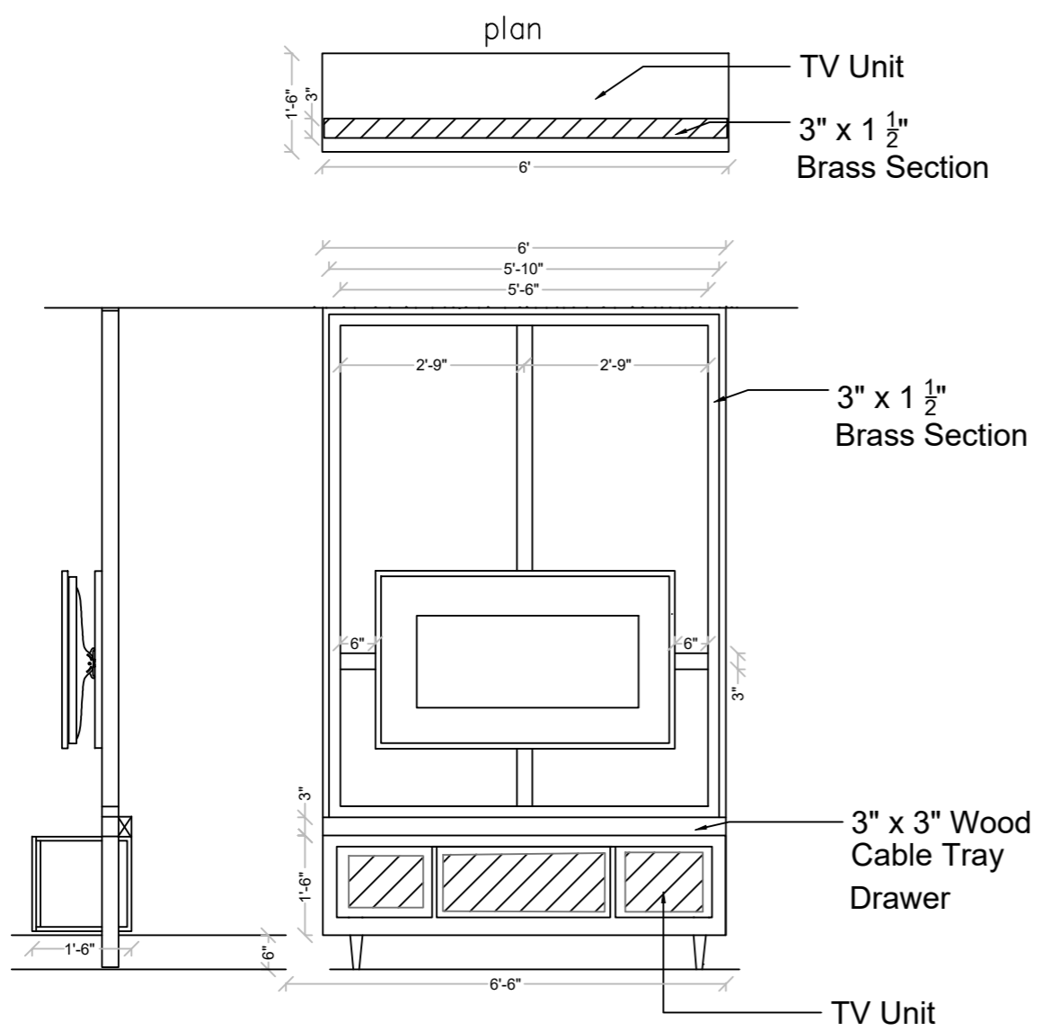
TV Unit , Hallway side
