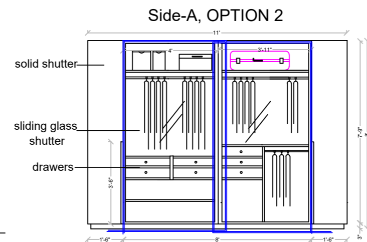
ELEVATIONS SON'S WARDROBE 1st FLOOR, Exterior
