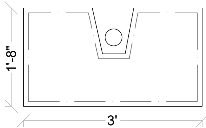
drawer plan
